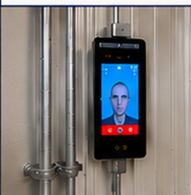
FACE RECOGNITION
